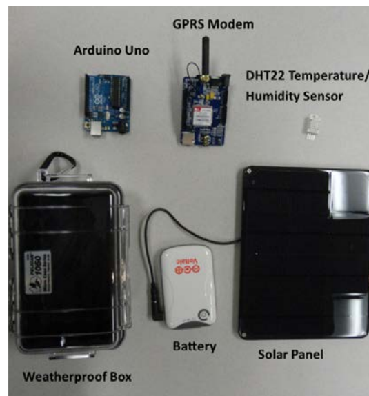
Figure 2. Arduino, solar panel, battery, sensor, and GPRS modem
